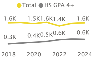
Frosh Applications
