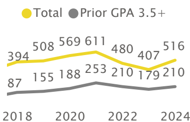
Transfer Applications
